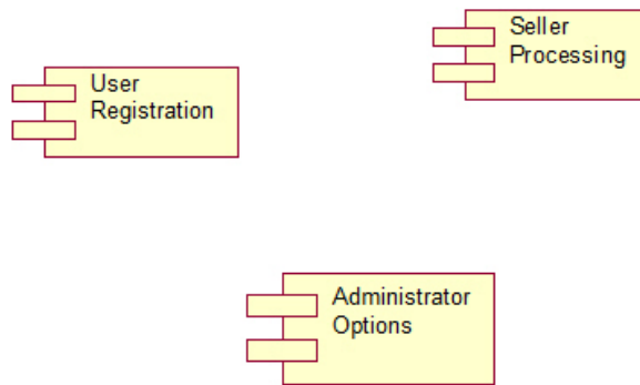
( http://www.startertutorials.com/uml/wp-content/uploads/2013/11/OBS-Component-Diagram-Business-Classes1.jpg )
