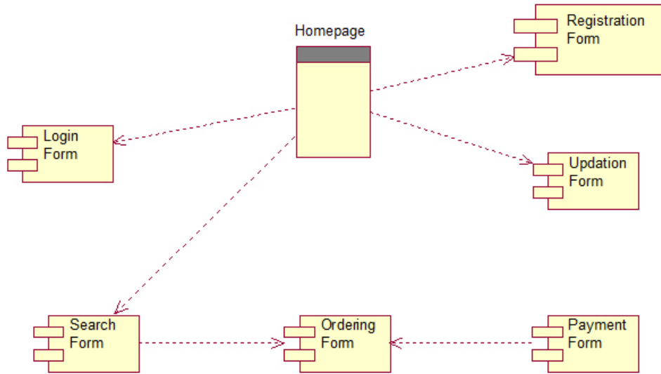
( http://www.startertutorials.com/uml/wp-content/uploads/2013/11/OBS-Component-Diagram-View-Classes.jpg )
